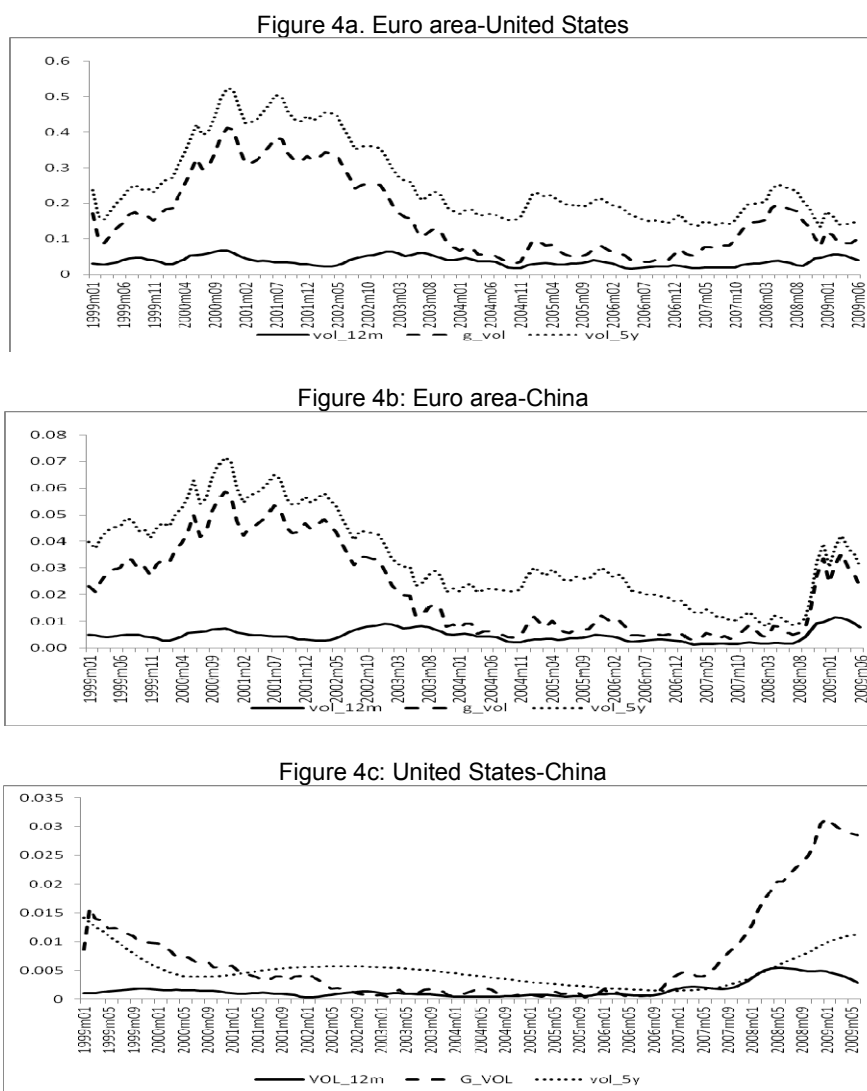
Figure 4. Evolution of the exchange rate volatility measures by country pair
