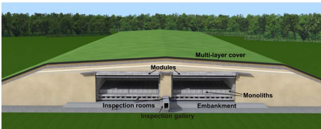
Figure 1.3: Overview of the disposal concept (ONDRAF/NIRAS 2011a)
