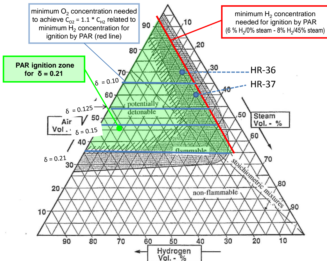
Fig. 0-4: Flammability limit of the H_2 - O_2 - H_2O system for different dilution ratios
