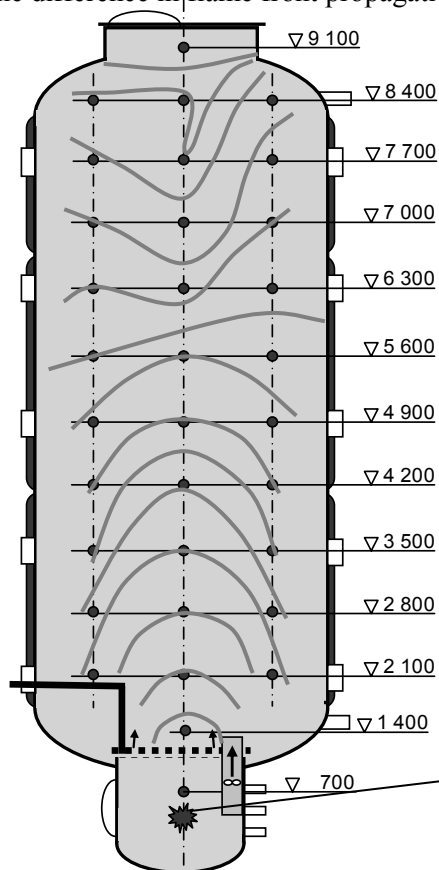
Fig. 5-2: Test without steam: Flame front propagation as isochrones
