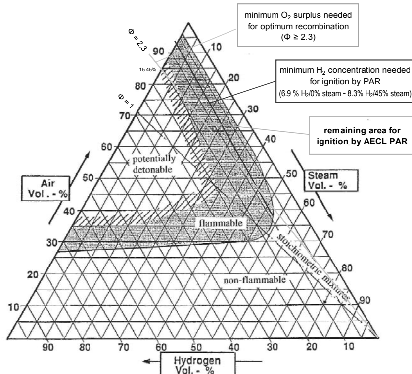
Fig. 5-5: Ternary diagram (example): Area of possible ignition by PAR (green shaded), resulting from HR test findings
