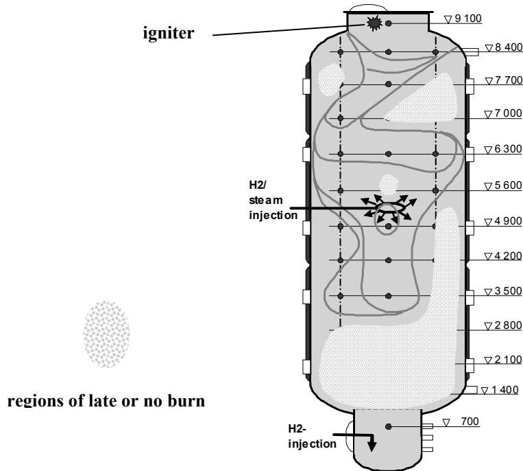
Fig. 5-4: Flame front propagation as isochrones: Test with lean mixture at vessel bottom; downward burn direction
