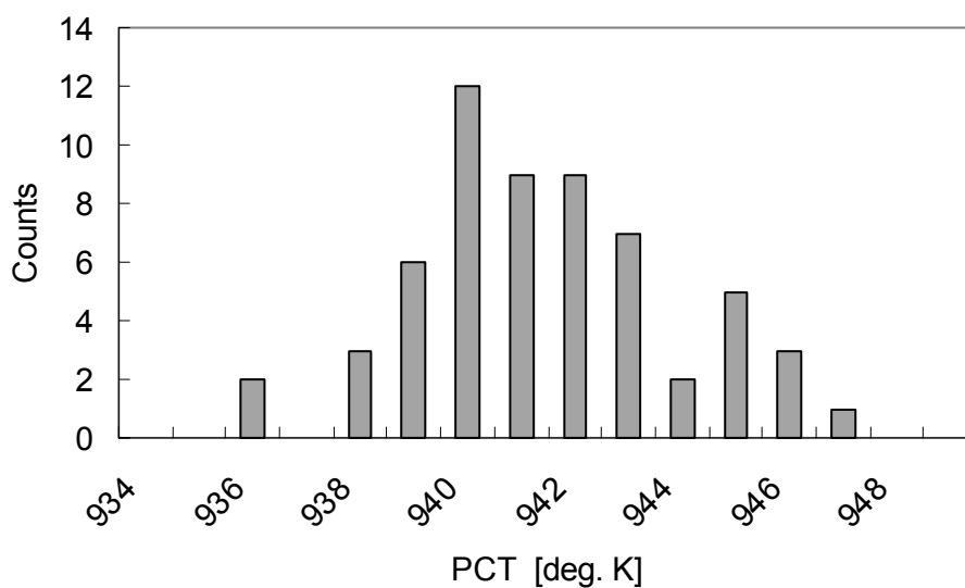
Figure 6-11. Histogram for small-break LOCA PCT at 104.5% power
