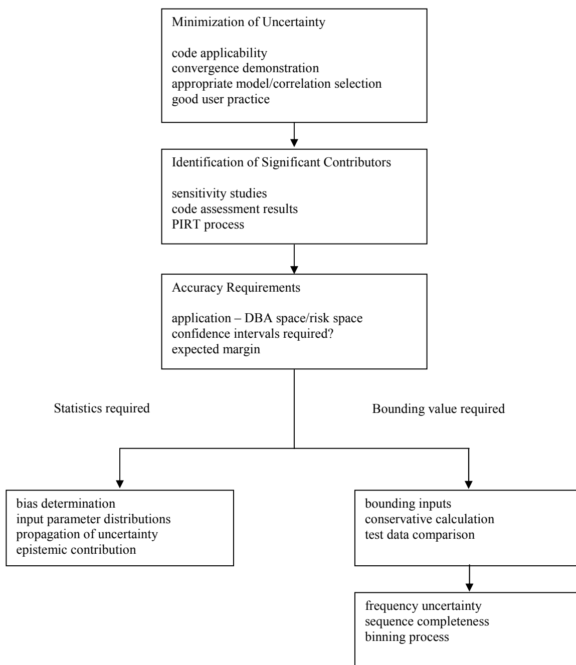
Figure 3-2. Schematic of Uncertainty Quantification Process
