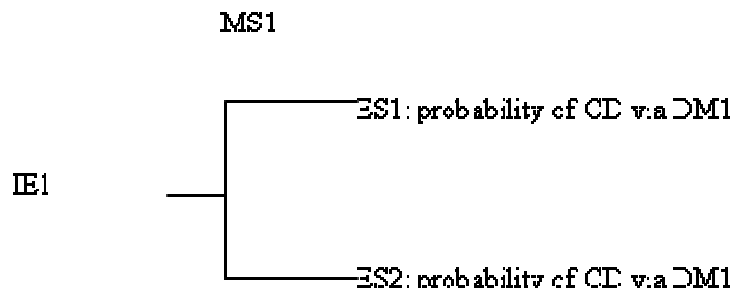
Figure 5-4. Reduced risk space for the example safety inquiry
