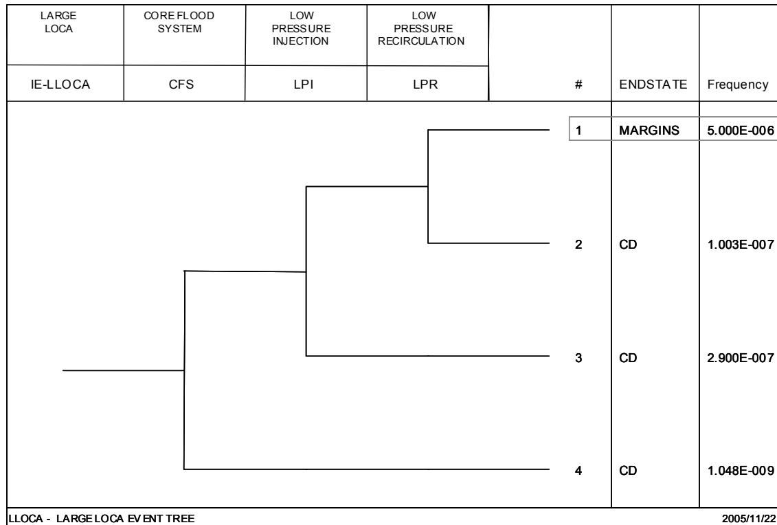
Figure 6-2. Large LOCA event tree for NPSH margin calculation
