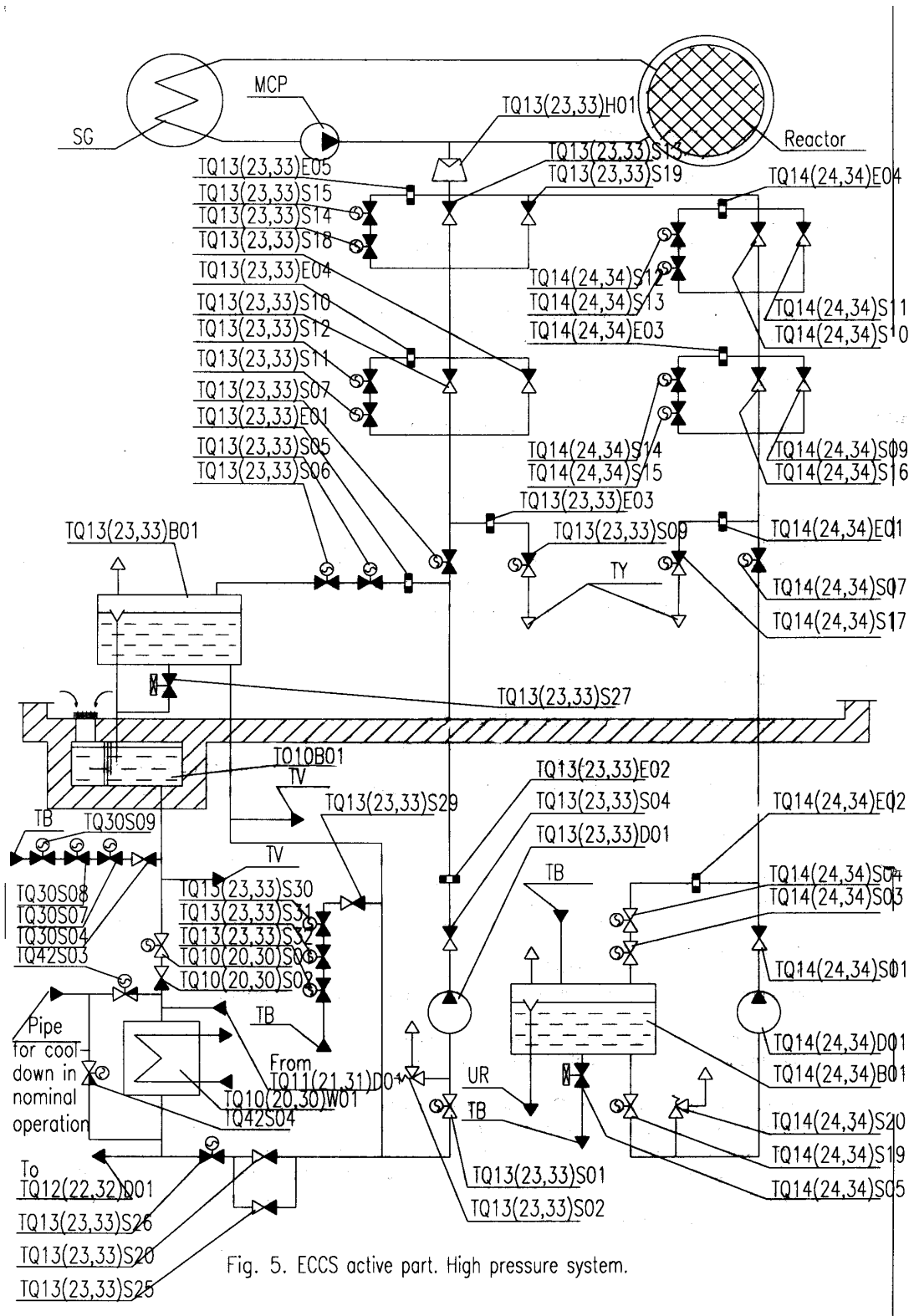
Figure 5: ECCS active part. High pressure System
