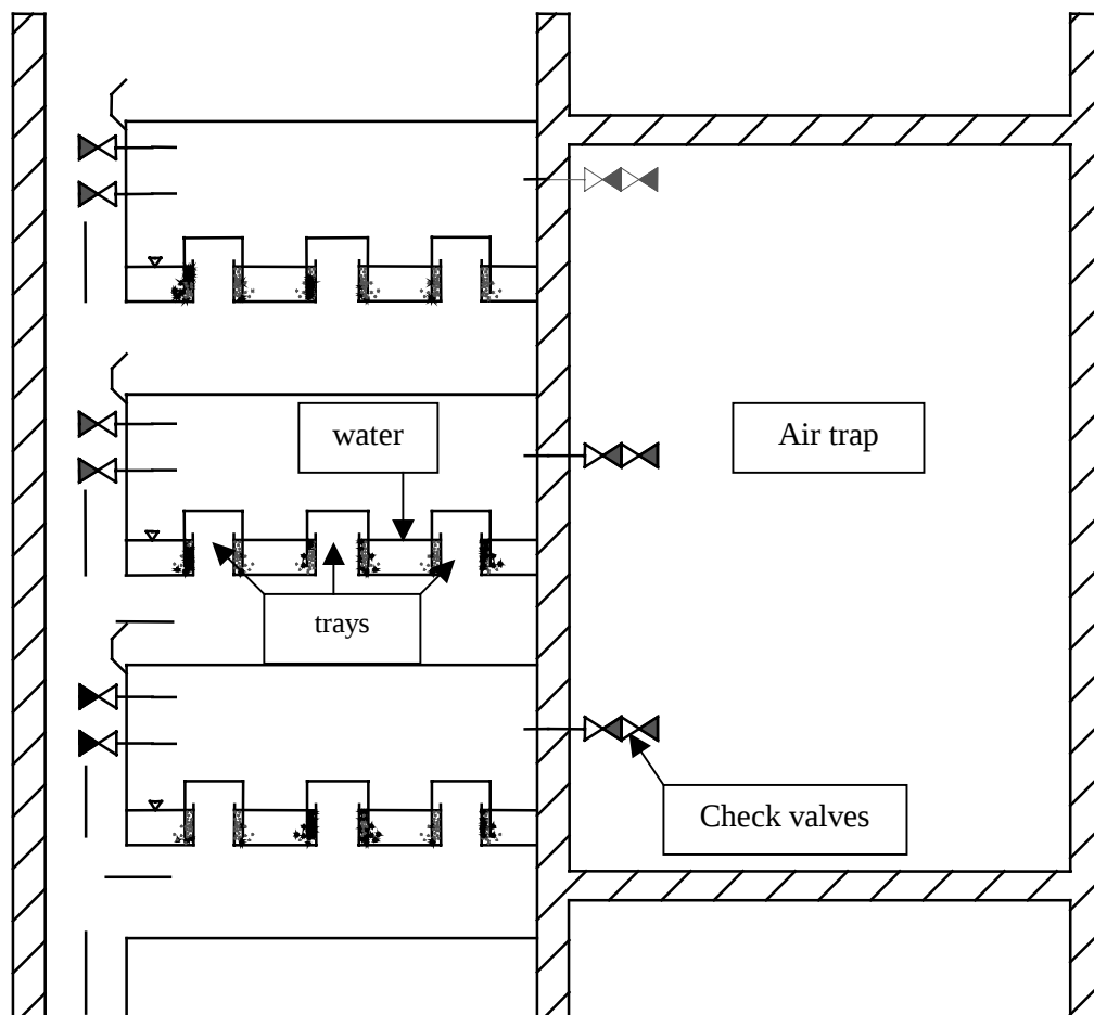
Fig.7. Schematic diagram of the bubbler condenser (3 out of 12 floors). (Ref: Rypar, O.:Barbotážní kondenzace páry, Revision 0, December 1998, Archive: MPOTH03-ÚJV-1998-12-006)
