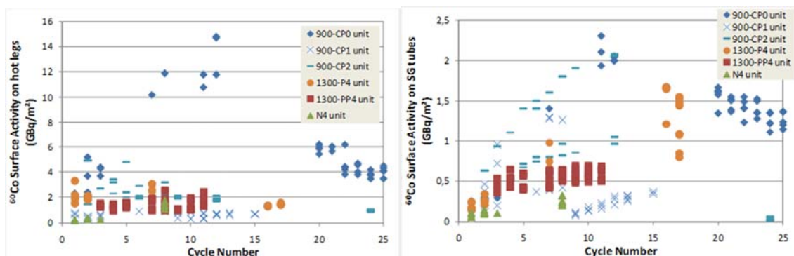
Figure 39: Evolution of ^{60}\text{Co} deposited activities on hot legs (39a) and steam generator tubes (39b)
