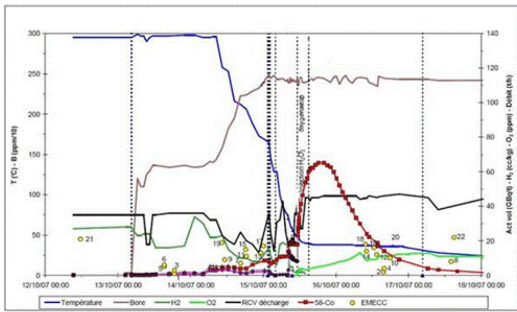
Figure 38: Measurement point localisation during shutdown
