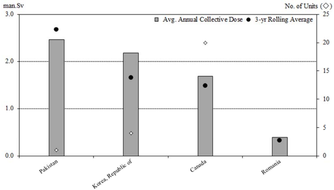
Figure 6: 2010 PHWR average collective dose per reactor by country (man-Sv/reactor)
