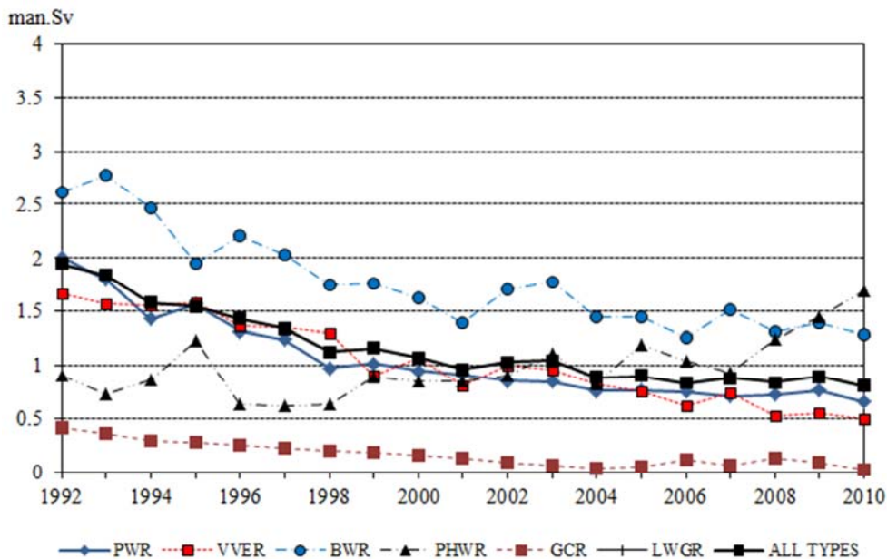
Figure 2: Three-year rolling average per reactor for all operating reactors included in ISOE by reactor type, 1992-2010 (man-Sv/reactor)
