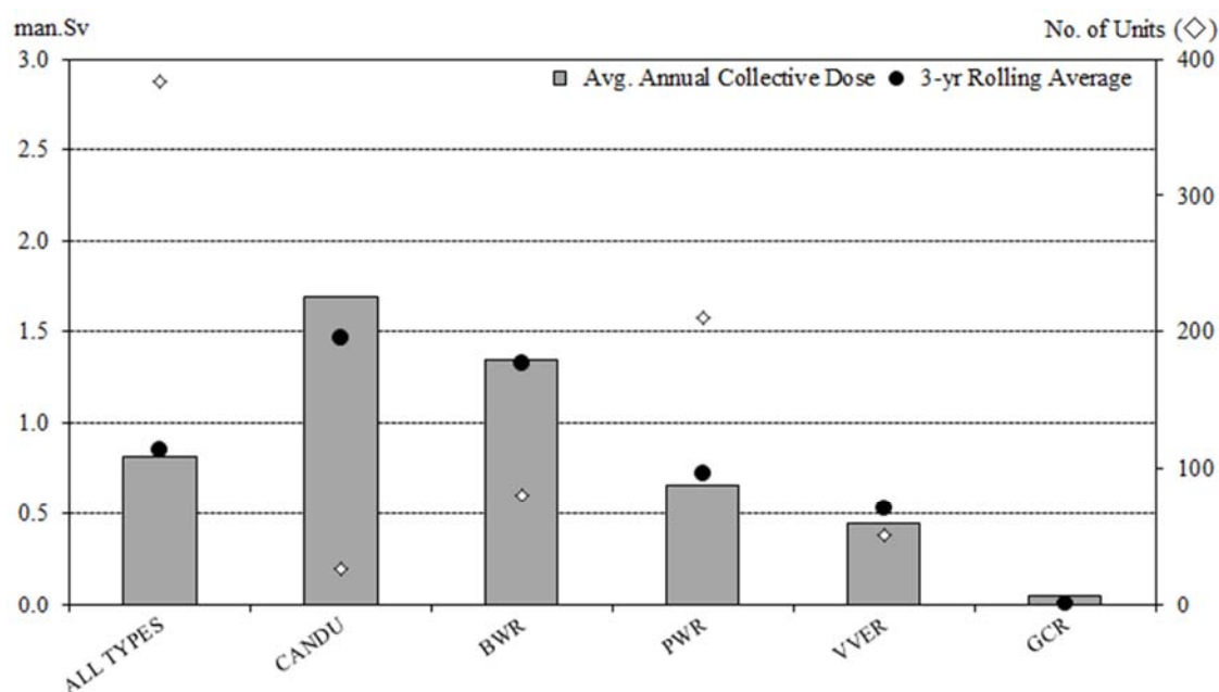
Figure 7: 2010 average collective dose per reactor by reactor type (man.Sv/reactor)
