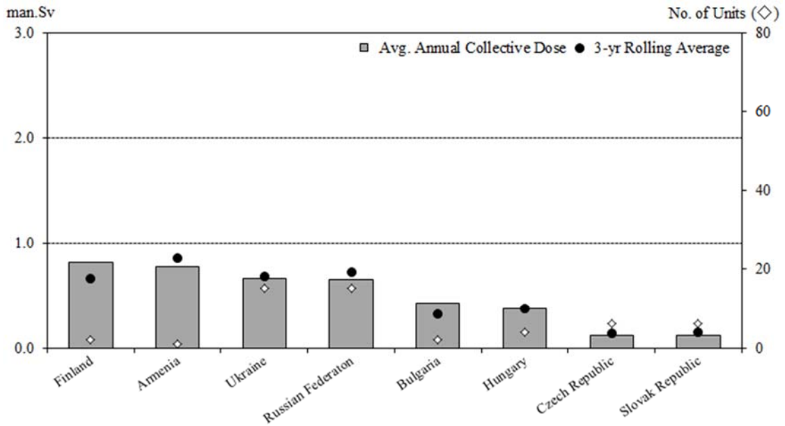
Figure 4: 2010 VVER average collective dose per reactor by country (man-Sv/reactor)
