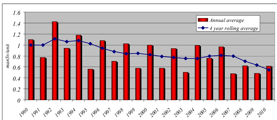
Collective dose: Annual and four-year rolling average in Finnish NPPs
