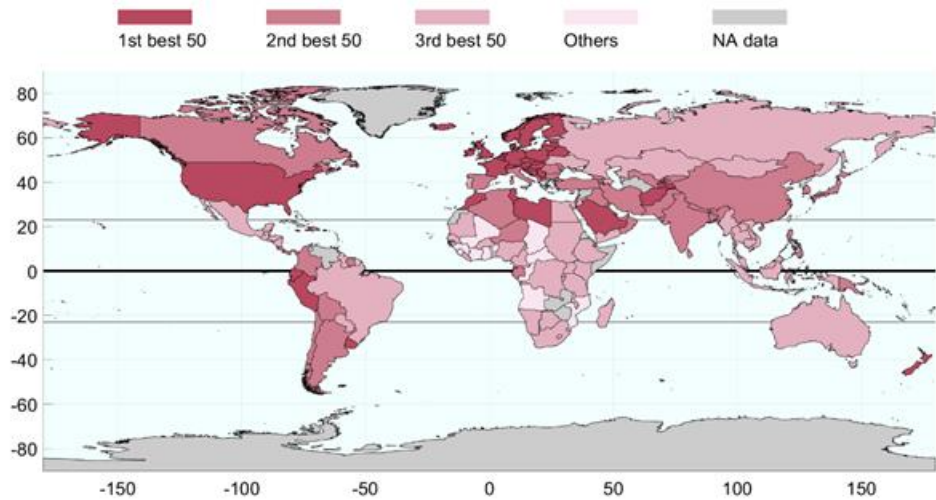
Figure 10. Global distribution of wildfire risk
