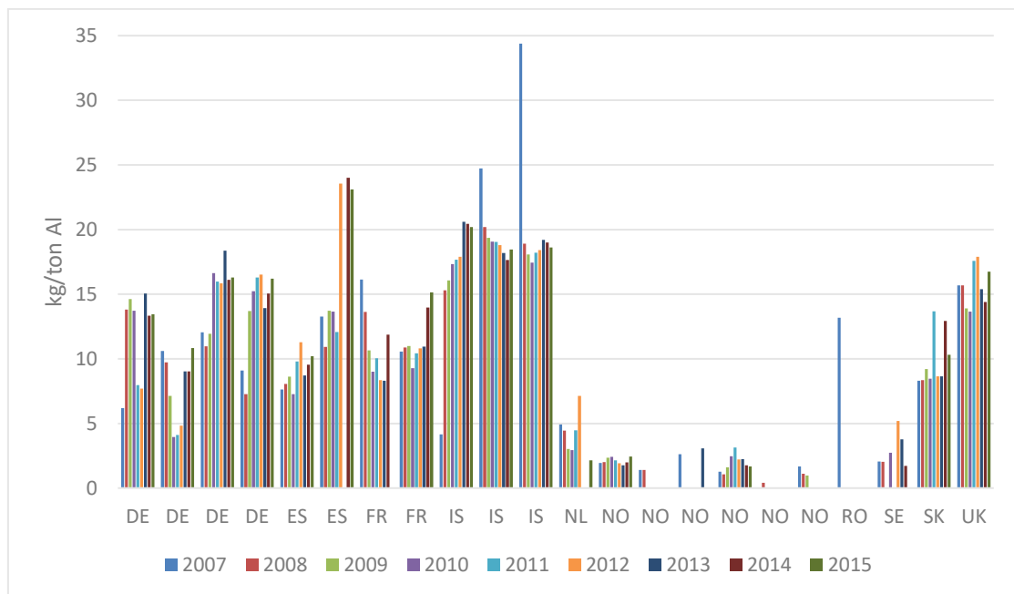
Figure 2.3. SO 2 emissions per unit of production in primary aluminium plants in the EU
