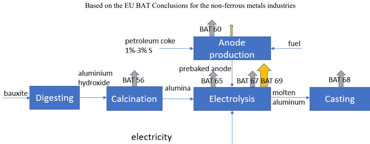
Figure 2.8. Simplified representation of the aluminium production based on pre-baked anodes
