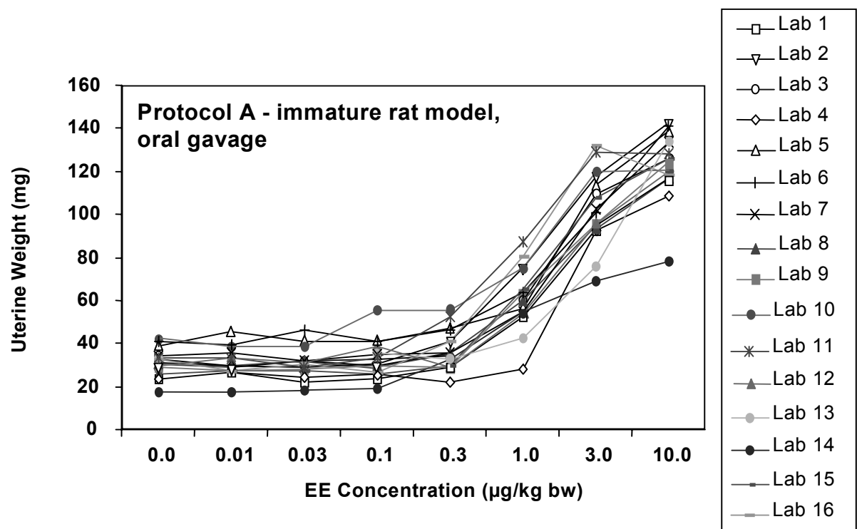
Figure 3. Responses of blotted uterine weight to doses of 17 \alpha -ethinyl estradiol (EE) following the four protocols in the validation work.
