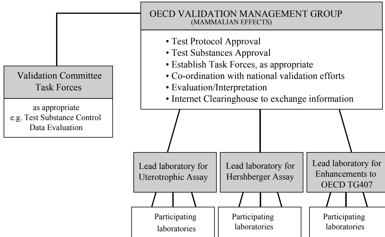
Figure 2. Schematic Diagram to Describe the Role and Structure of the OECD Validation Management Group
