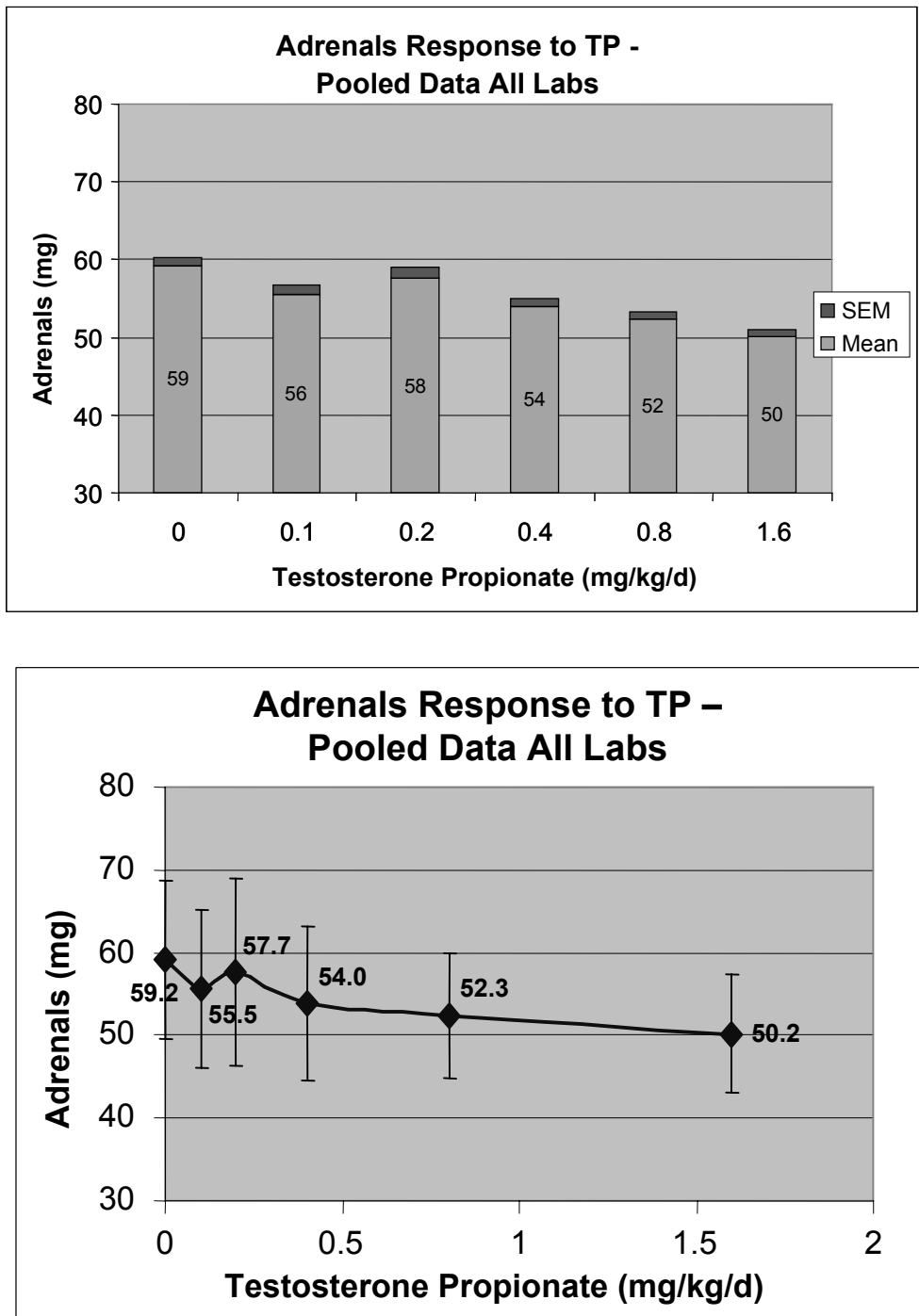
Figure 28. The response of adrenal weights using the mean of pooled data to increasing doses of testosterone propionate (TP) (sc). The top graph uses the standard error of the mean, which responds to sample size. The bottom graph uses the standard deviation from the pooled data. Note the reduced scale of the y-axis in both graphs. This incorporates significant laboratory variability and does not solely reflect the assay variability. Both graphs are plotted as the adrenal weights at necropsy.
