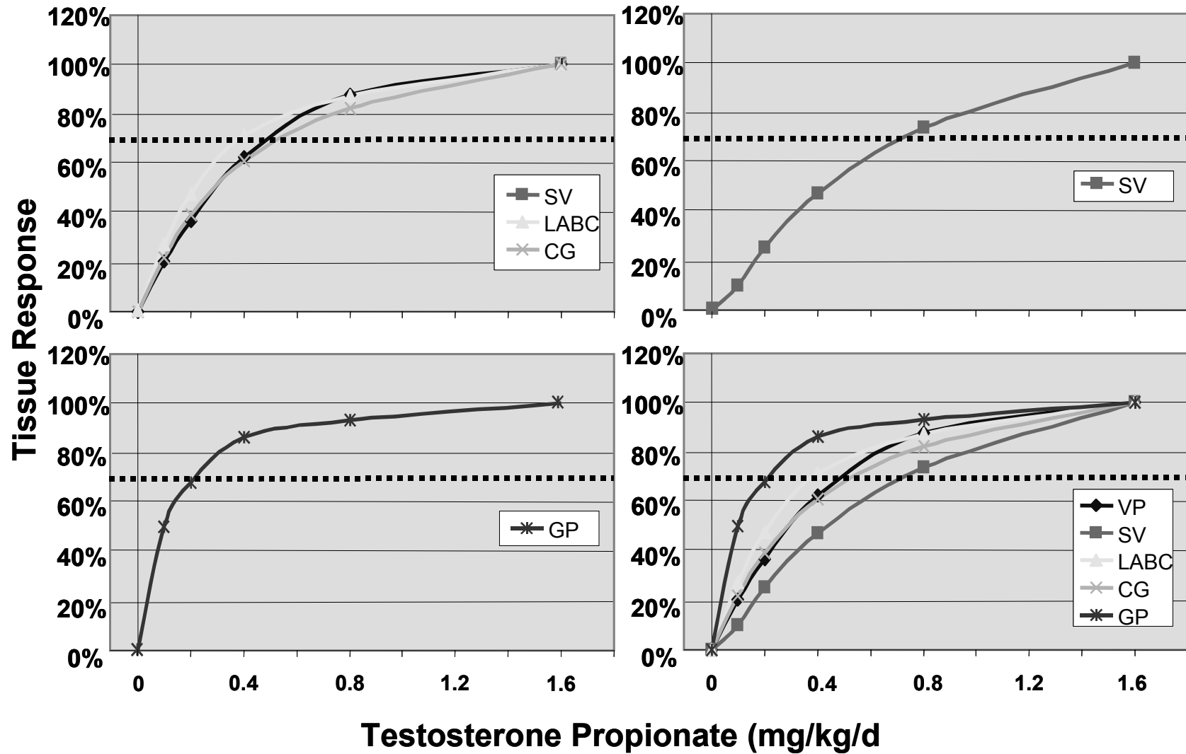
Figure 3. The three potential groups of male reproductive tissues are broken out using the normalized plot technique from Figure 2. Tissue abbreviations are also the same.
