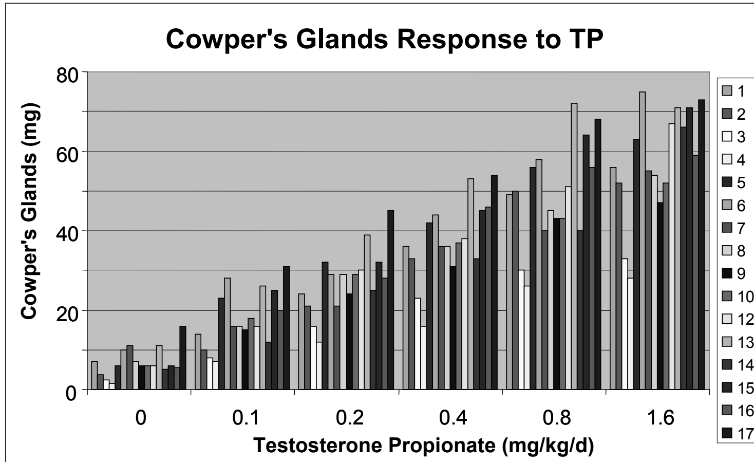
Figure 20. The individual responses of the mean of the Cowper's glands weights from each of 16 laboratories (1 laboratory, #11, administered micrograms rather than milligrams of TP) plotted as a bar graph.
