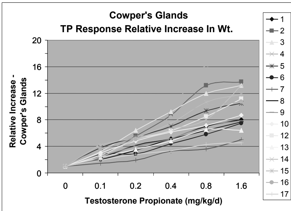
Figure 21. The individual responses of the mean of the Cowper's gland weights from each of 16 laboratories. The top graph is plotted as the absolute weight for each laboratory. The bottom graph is plotted as the relative increase in weight versus the control with the Cowper's glands increasing between 4- and 16-fold, depending upon the laboratory
