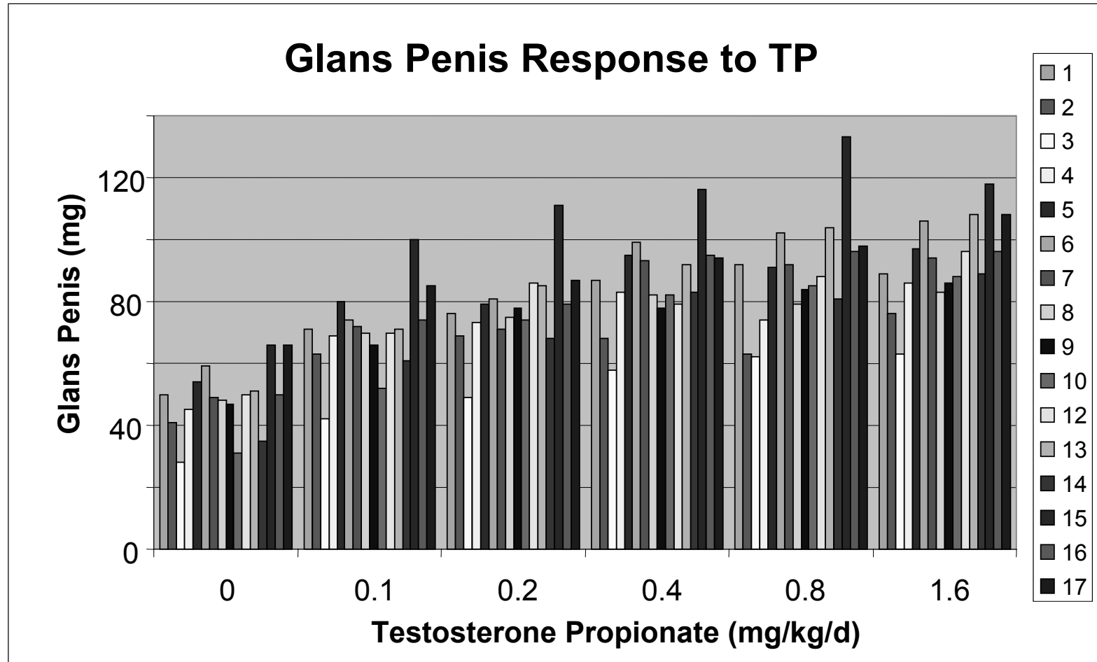
Figure 17. The individual responses of the mean of the glans penis weights from each of 16 laboratories (1 laboratory, #11, administered micrograms rather than milligrams of TP) plotted as a bar graph.
