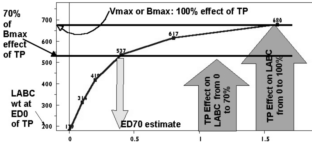
Figure 1. The x-axis is the testosterone propionate dose in mg/kg/d administered subcutaneously. The y-axis is the weight of the levator ani/bulbocavernosus muscle complex (LABC). This curve and markings demonstrate how an ED70 would be estimated from the data as 70% of the maximum effect as the dose response curve plateaus.
