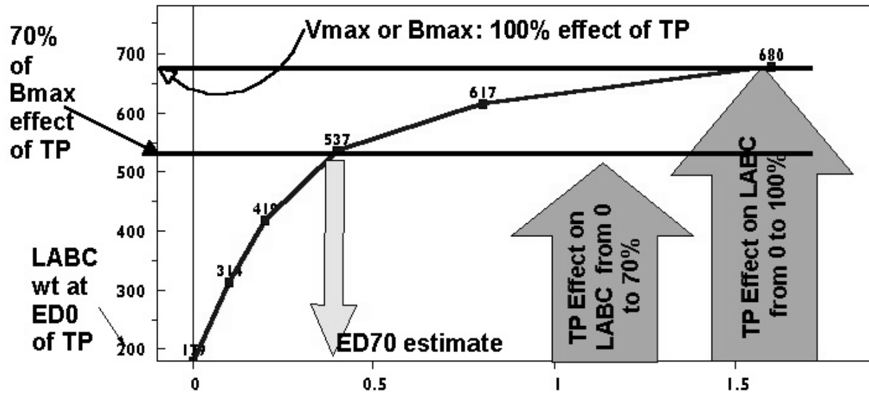
Figure 3. The x-axis is the testosterone propionate dose in mg/kg/d administered subcutaneously. The y-axis is the weight of the levator ani/bulbocavernosus muscle complex. This curve and markings demonstrate how an ED70 would be estimated from the data as 70% of the maximum effect as the dose response curve plateaus.
