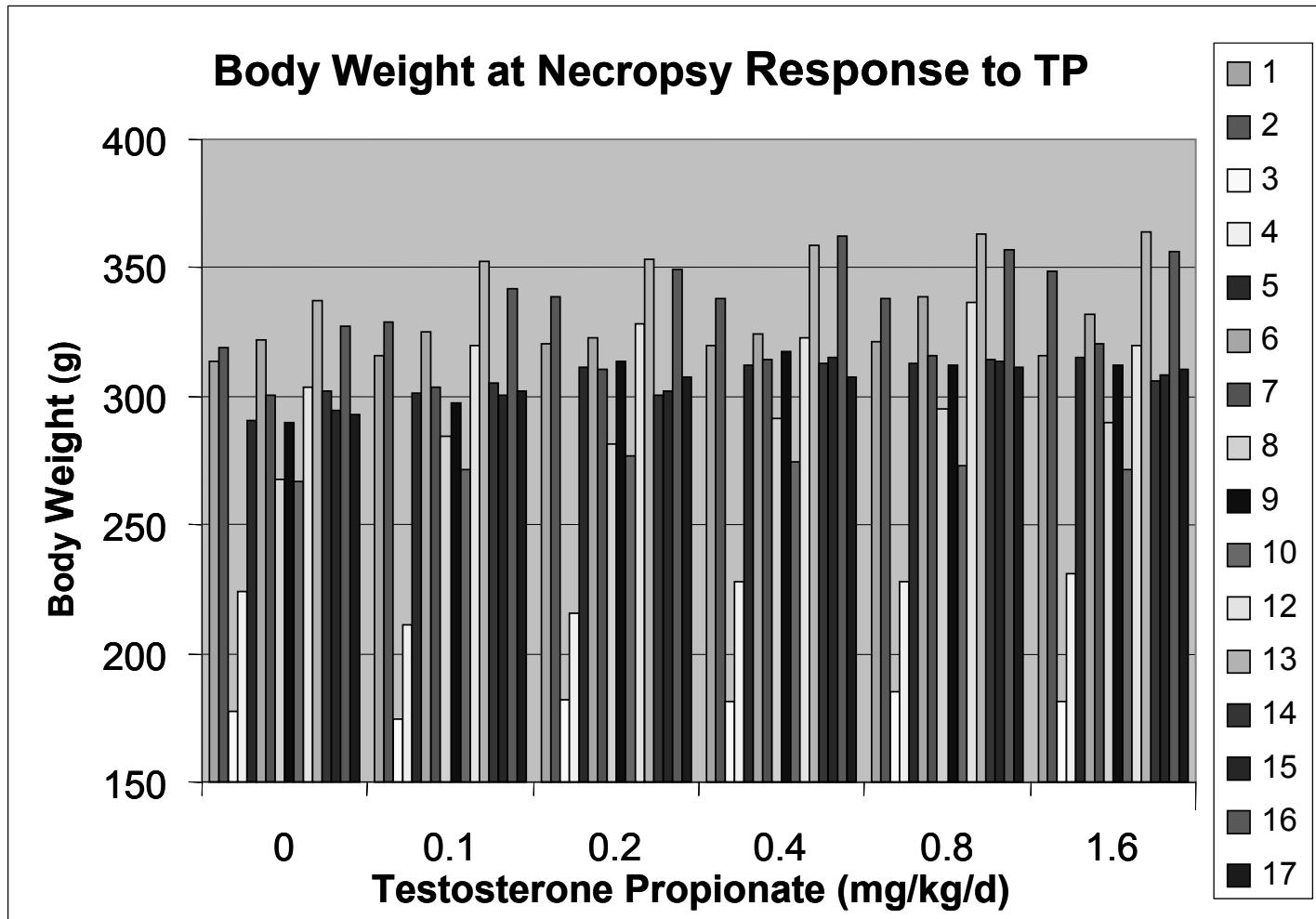
Figure 22. The individual responses of the mean of the body weights from each of 16 laboratories (1 laboratory, #11, administered micrograms rather than milligrams of TP) plotted as a bar graph.
