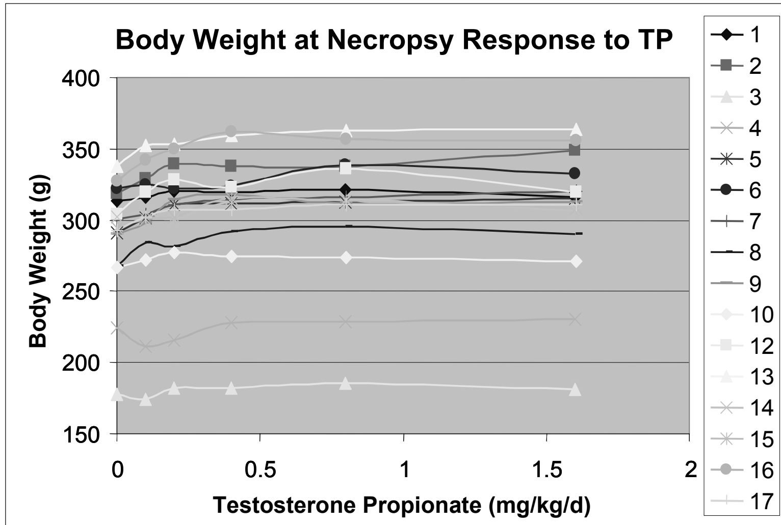
Figure 23. The individual responses of the mean of the necropsy body weights from each of 16 laboratories in response to increasing TP injections.
