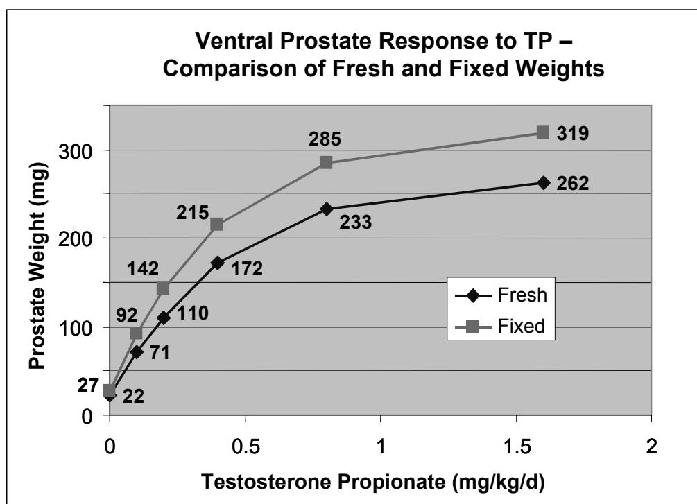
Figure 7. Comparison of pooled means of fresh prostates (16 labs) and fixed prostates weighed after 24 hours of fixation (15 labs). Upper graph is a bar graph comparison, and lower graph is a linear line graph comparison.
