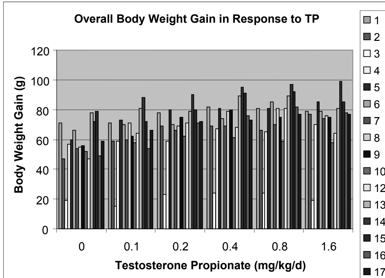
Figure 25. The individual responses of the mean gain in body weights from each of 16 laboratories for each dose group of TP. Note that laboratory 3 had the lowest starting body weights (see Figure 23) and here has the lowest body weight gains.
