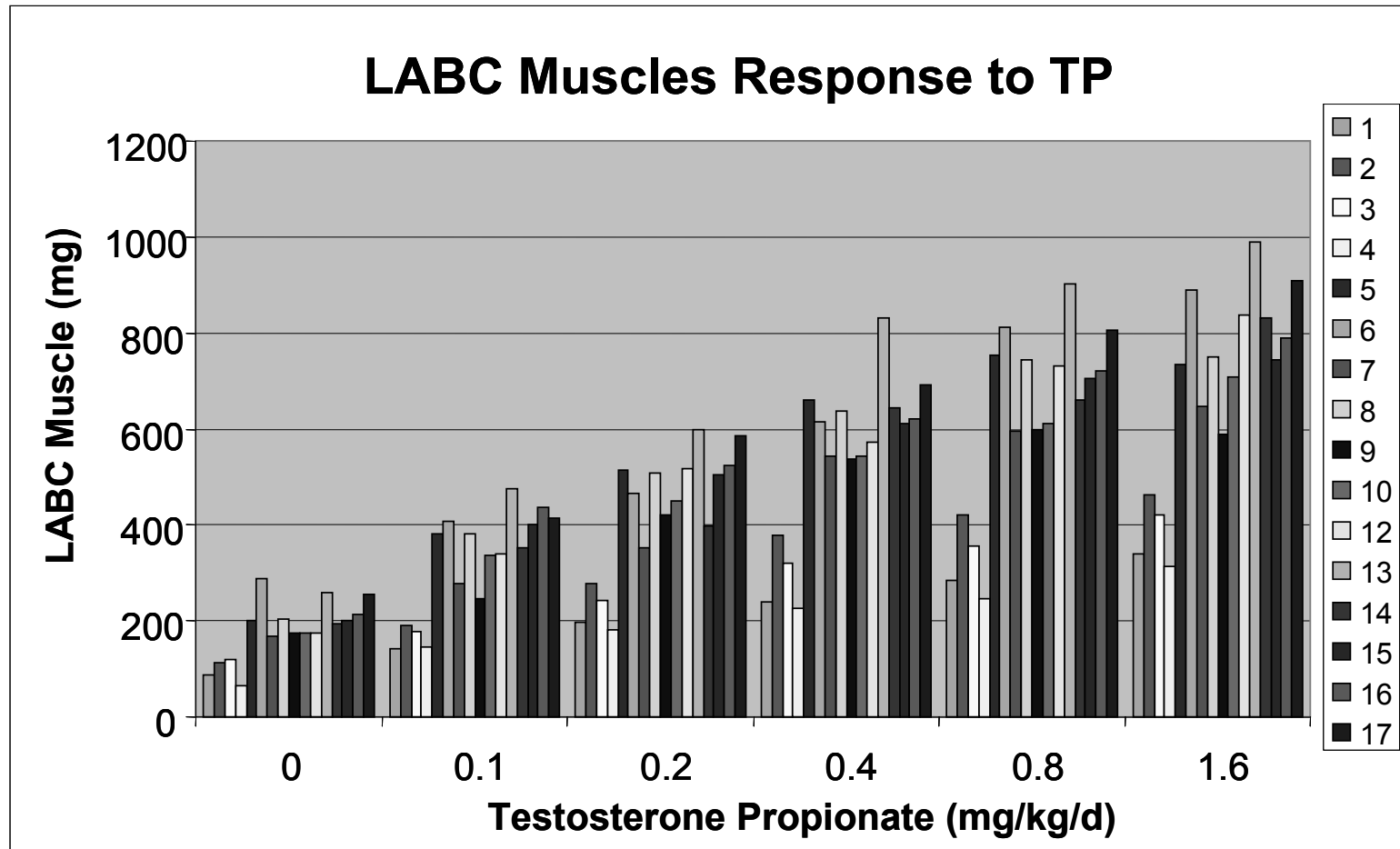
Figure 14. The individual responses of the mean of the LABC weights from each of 16 laboratories (1 laboratory, #11, administered micrograms rather than milligrams of TP) plotted as a bar graph.
