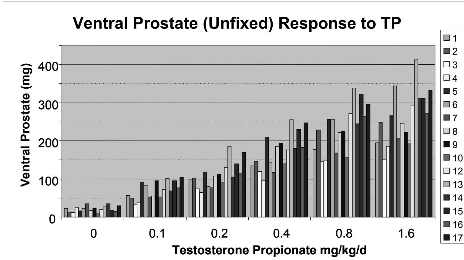
Figure 5. The individual responses of the mean of the fresh, unfixed ventral prostate weight from each of 16 laboratories (1 laboratory, #11, administered micrograms rather than milligrams of TP) plotted as a bar graph.
