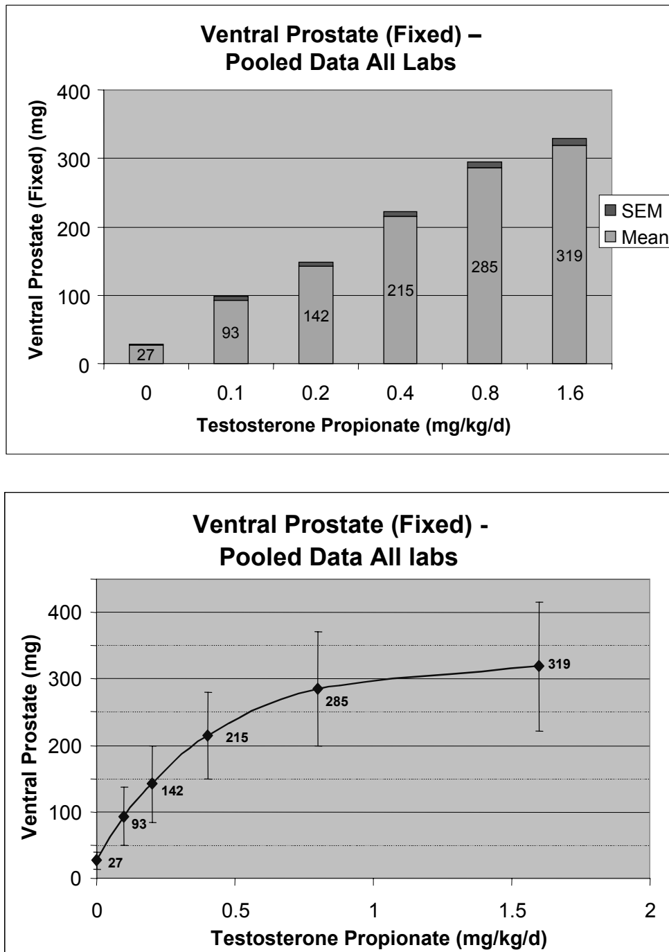
Figure 8. The response of the fixed ventral prostate (fixed after dissection and weighed 24 hours later) using the mean of pooled data from 15 laboratories (one laboratory did not fix and weigh the prostate) in to increasing doses of testosterone propionate (TP) (sc). The top graph uses the standard error of the mean, which responses to sample size (90 samples per dose in this case). The bottom graph uses the standard deviation from the pooled data. This incorporates significant laboratory variability and does not solely reflect the assay variability. Both graphs are plotted as the weight of fixed prostate.
