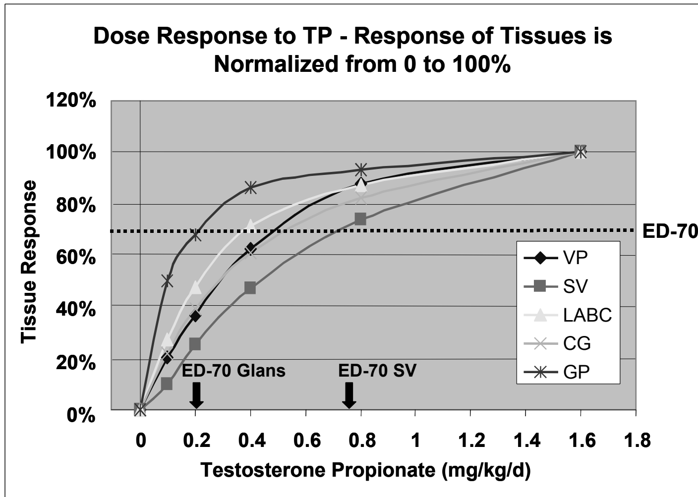
Figure 2. The pooled data across 16 laboratories for each tissue has been normalized so that the control value = 0% and the maximum reached at 1.6 mg/kg/d testosterone propionate (TP) = 100%. The differences between tissues in how rapidly a tissue reaches its maximum is then illustrated, e.g., glans penis first and seminal vesicles last. VP = ventral prostate; SV = seminal vesicles and coagulating glands; LABC = levator ani/bulbocavernosus muscle complex; CG = Cowper's glands; GP = glans penis.
