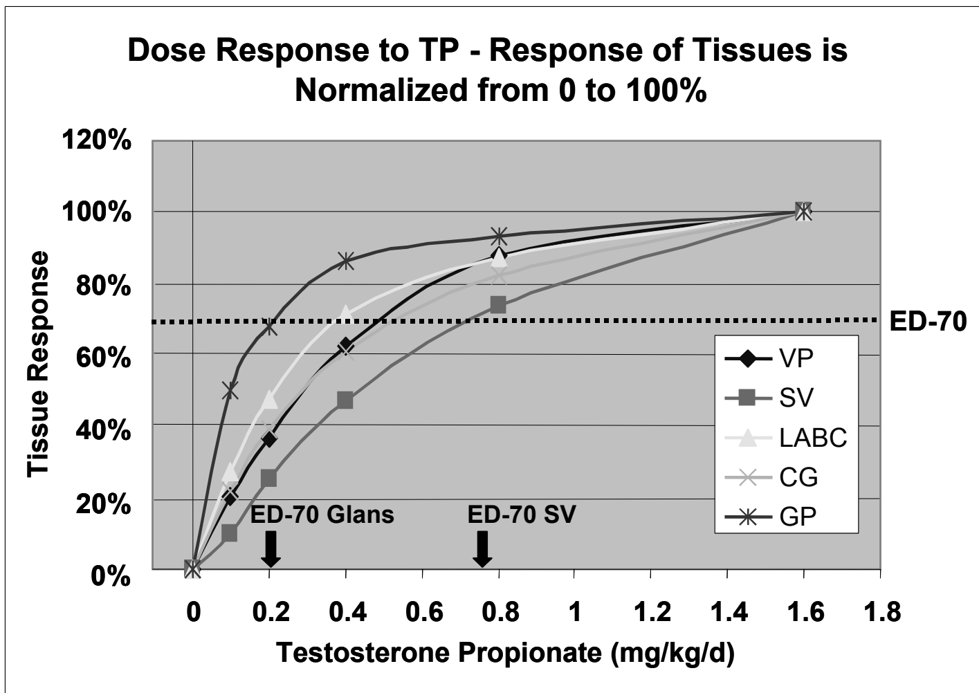
Figure 1. The pooled data across 16 laboratories for each tissue have been normalized so that the control value = 0% and the maximum reached at 1.6 mg/kg/d testosterone propionate (TP) = 100%. The differences between tissues in how rapidly a tissue reaches its maximum is then illustrated, e.g., glans penis first and seminal vesicles last. VP = ventral prostate; SV = seminal vesicles and coagulating glands; LABC = levator ani/bulbocavernosus muscle complex; CG = Cowper’s glands; GP = glans penis.
