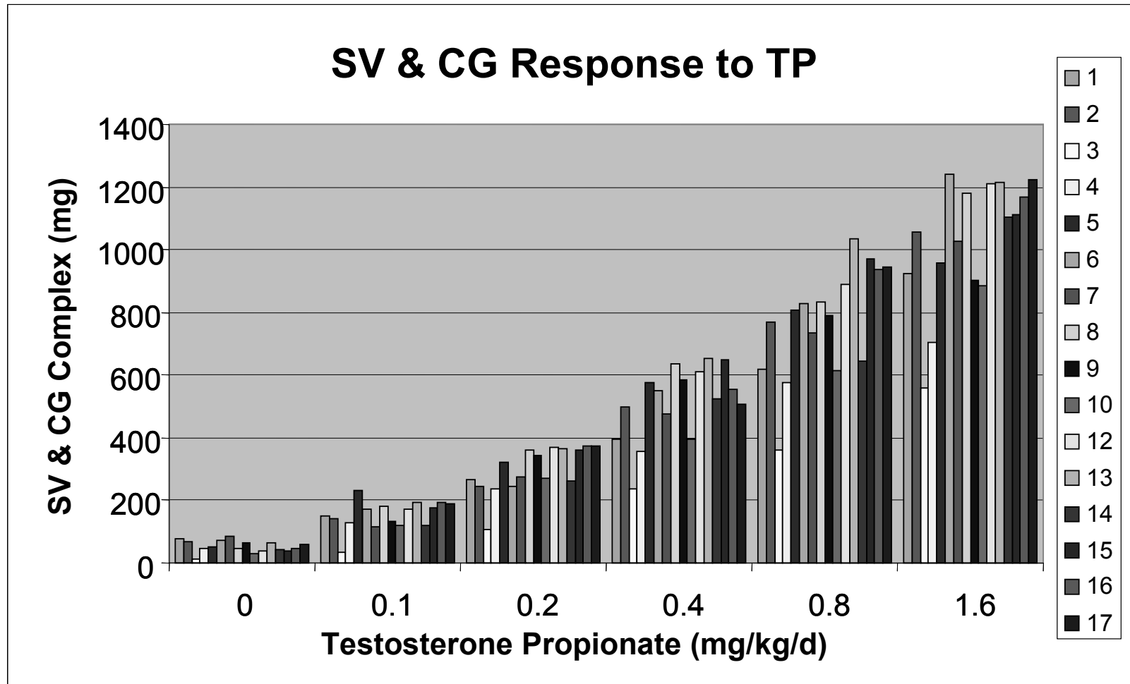
Figure 11. The individual responses of the mean of the seminal vesicle and coagulating gland weights from each of 16 laboratories (1 laboratory, #11, administered micrograms rather than milligrams of TP) plotted as a bar graph.
