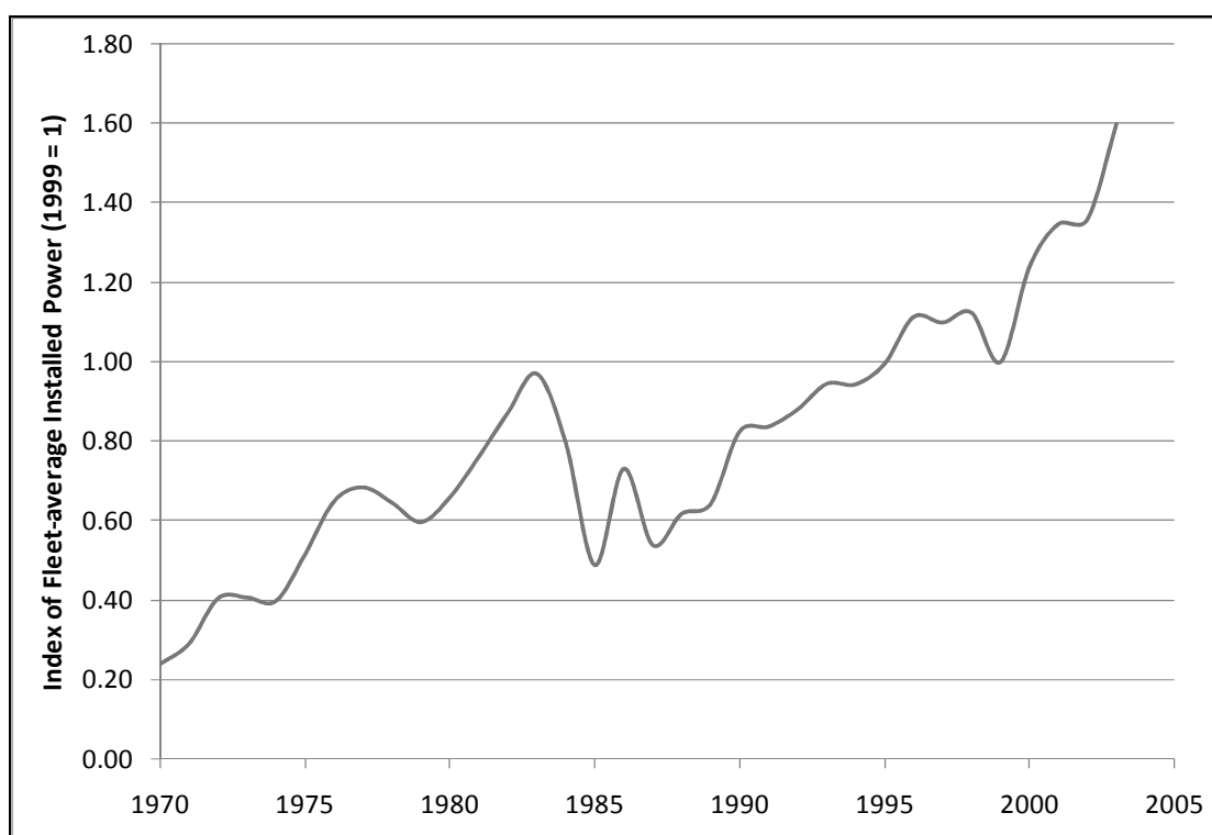
Figure 11. Average installed power (kW) for world-wide vessel fleet, 1970 - 2003
