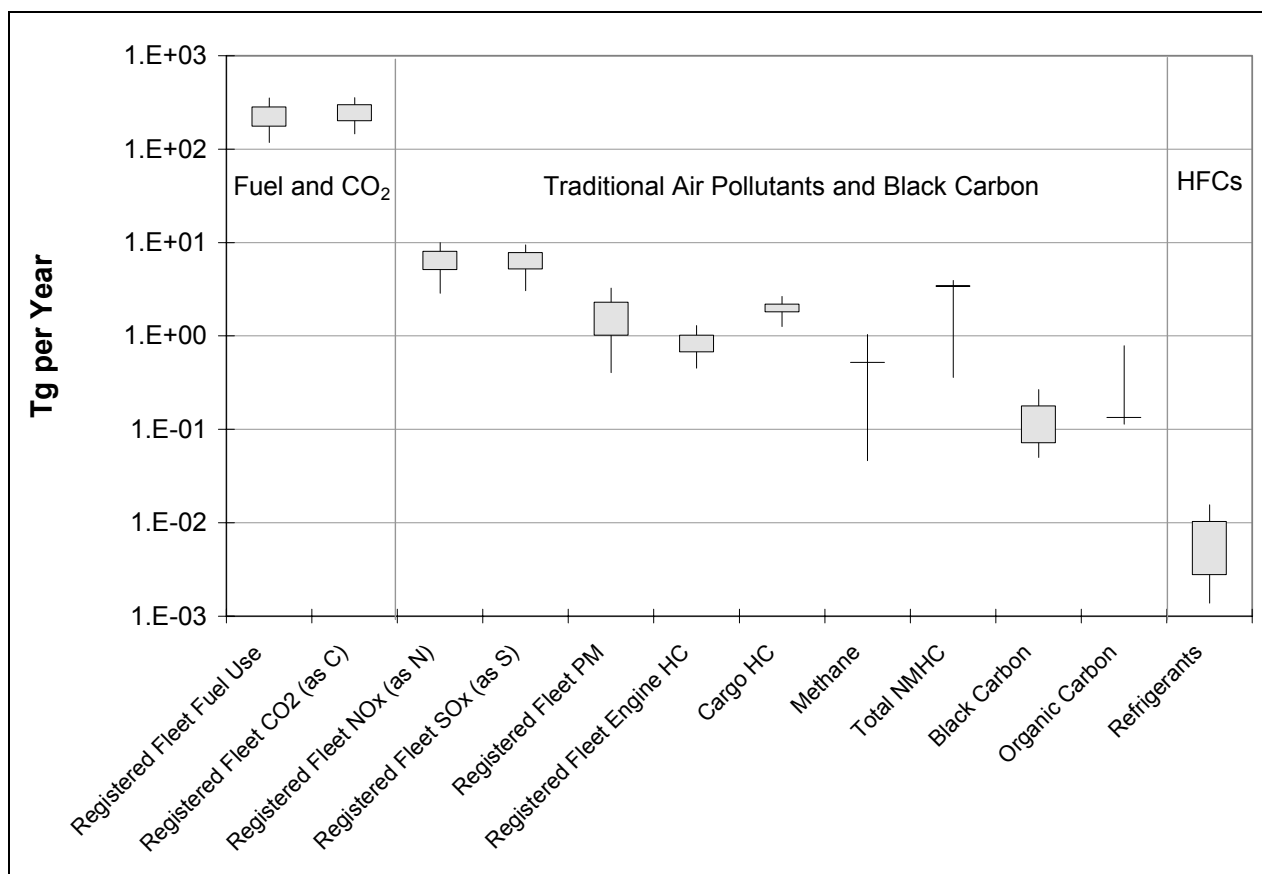
Figure 14. Summary of estimated ranges in global emissions from maritime shipping, 2002
