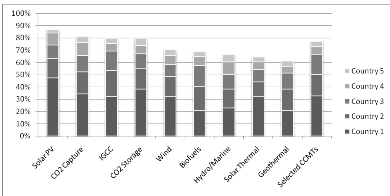
Figure 12. Proportion of patenting (CP) by the top 5 ranking inventor countries for each CCMT field, 1988-2007
