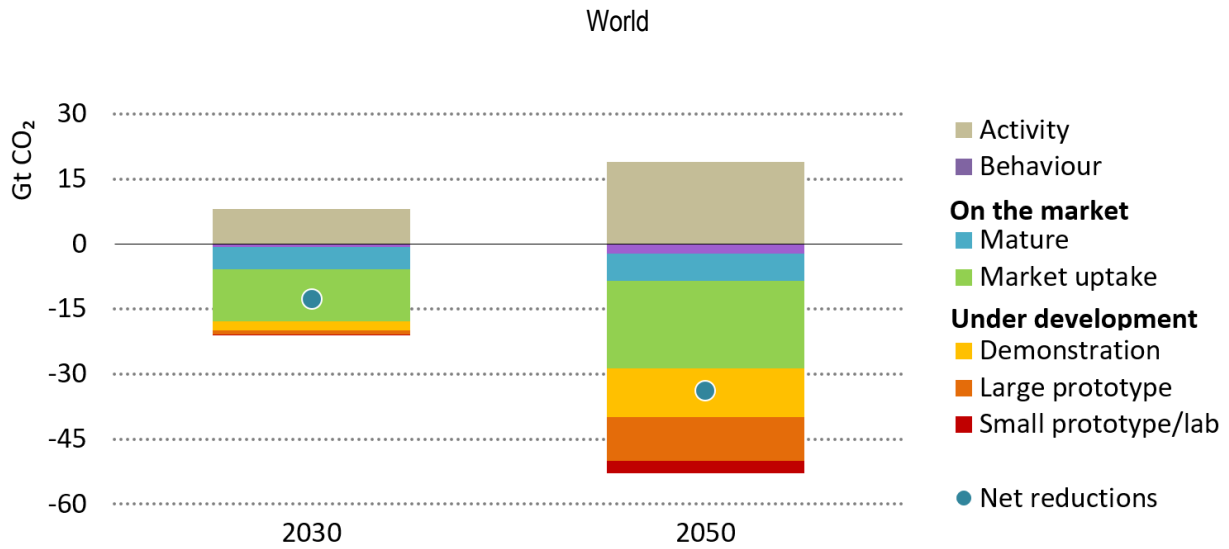
Figure 11. Clean technology innovations are critical for decarbonising buildings
