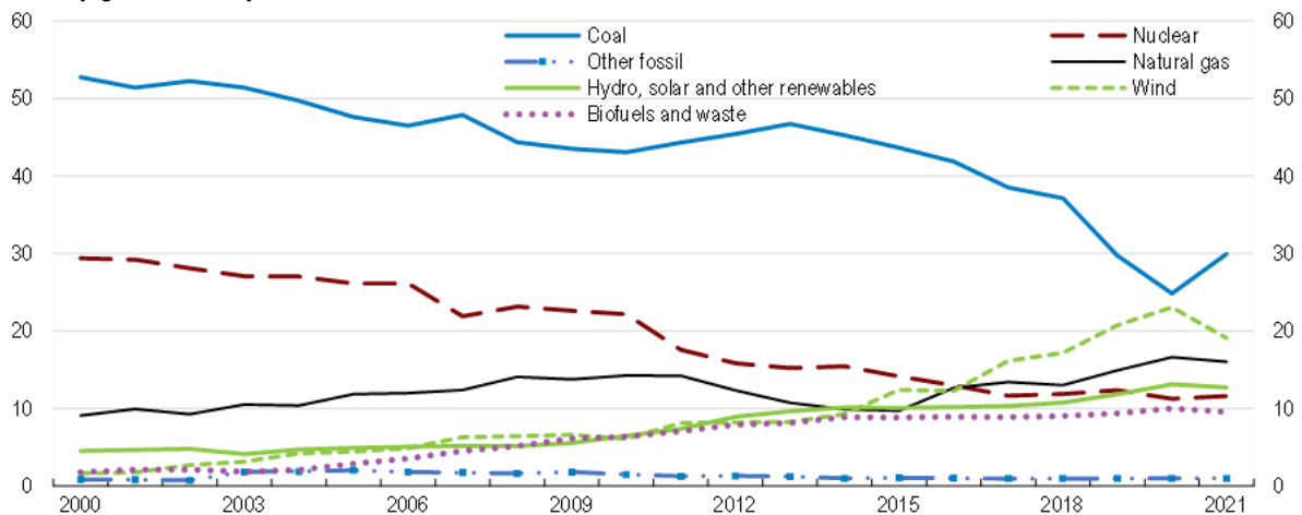
Figure 27. Coal uses for electricity generation steadily declined until 2020
