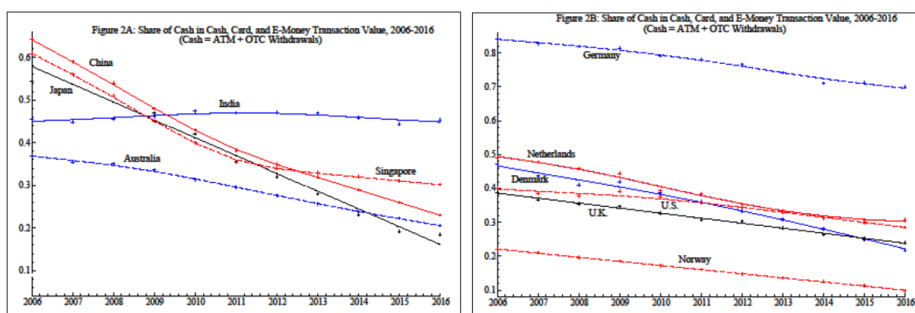
Figure 5. Share of Cash in Cash, Card and E-money transaction value in 11 countries, 2006-2016
