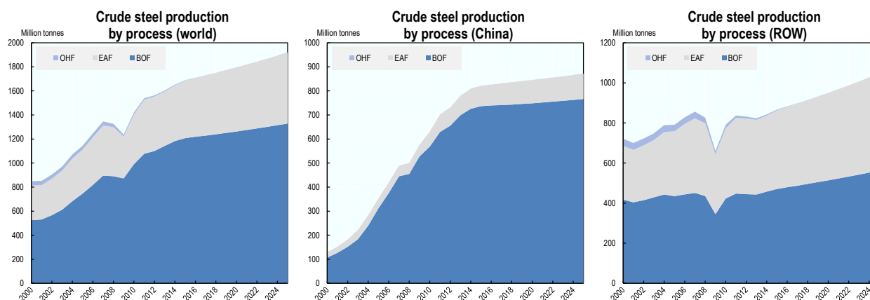
Figure 3. Global crude steel production by process (2000-2025)
