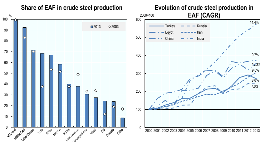
Figure 2. The development of EAF in crude steel production
