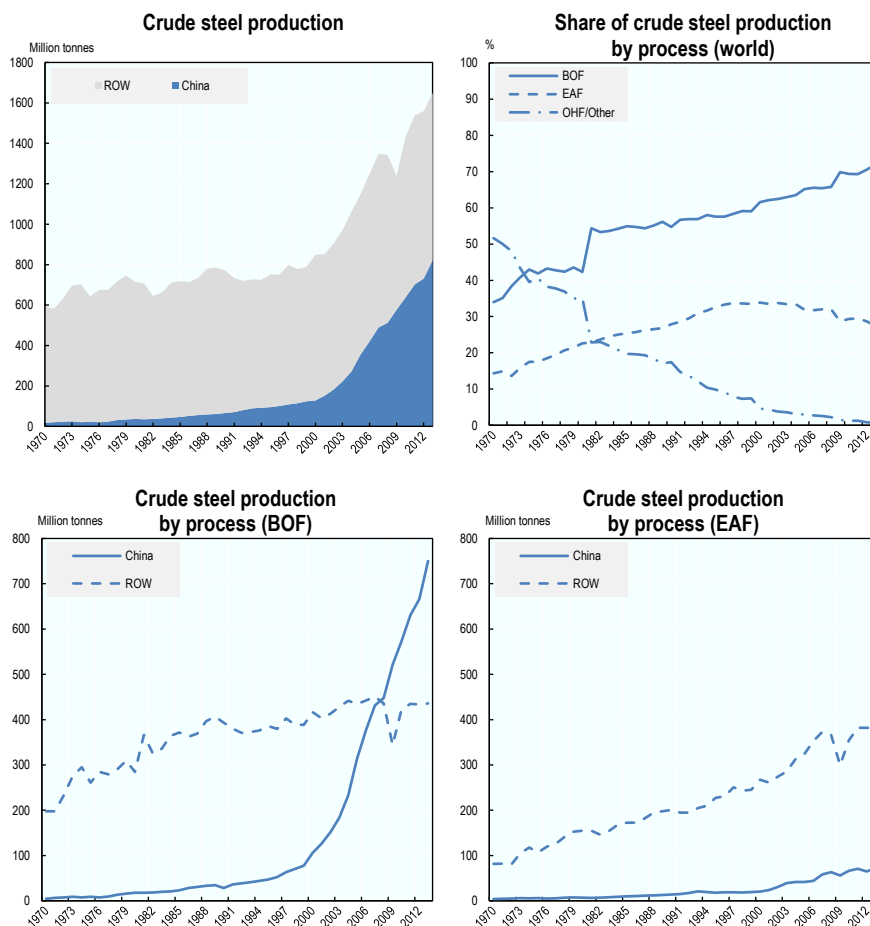
Figure 1. Crude steel production (1970-2013)
