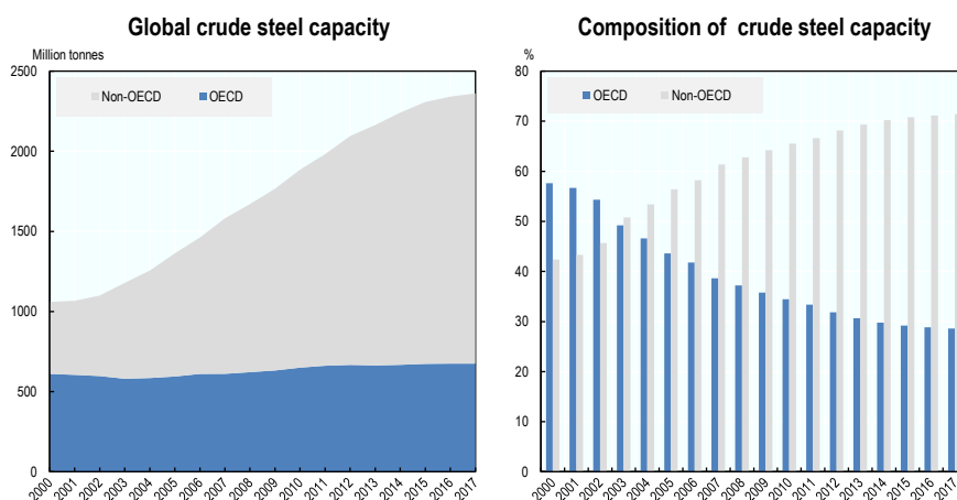
Figure 4. Global nominal crude steel capacity
