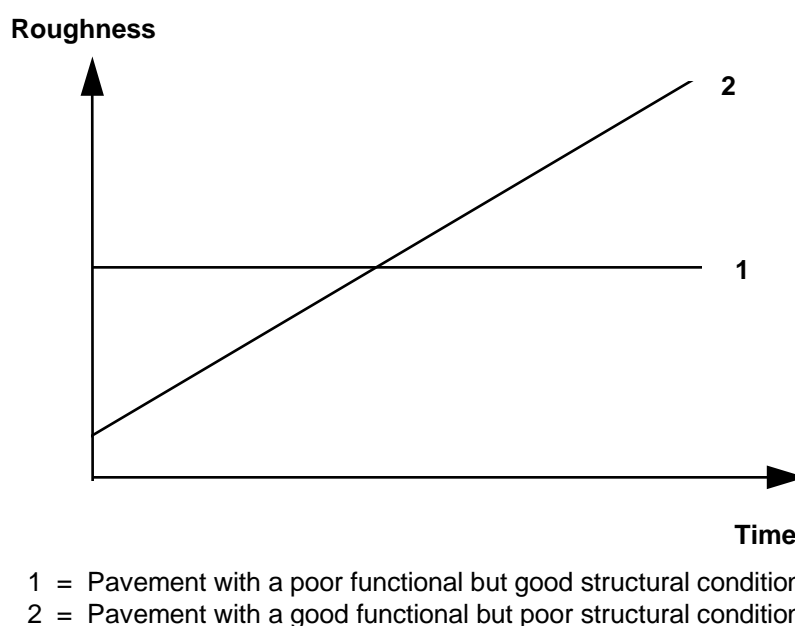
Figure II.2. Difference between “functional condition” and “structural condition”
