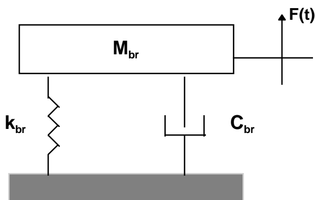
Figure III.3. Simplified vehicle-bridge dynamic model for short-span bridges
