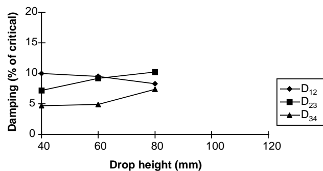
Figure IV.31. Damping ratio of a steel suspension: simultaneous axle drop
