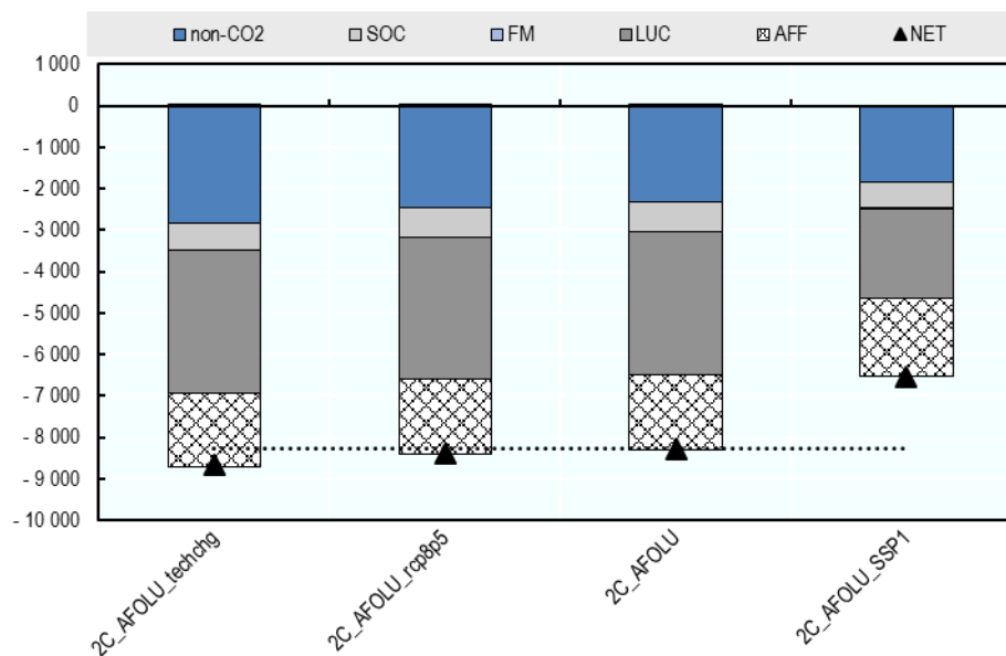
Figure 19. Mitigation (GtCO 2 eq) from the AFOLU-wide policy to assumptions about climate, technology, global coverage and socio-economic pathway, relative to the baseline in 2050, in relation to the 2°C target
