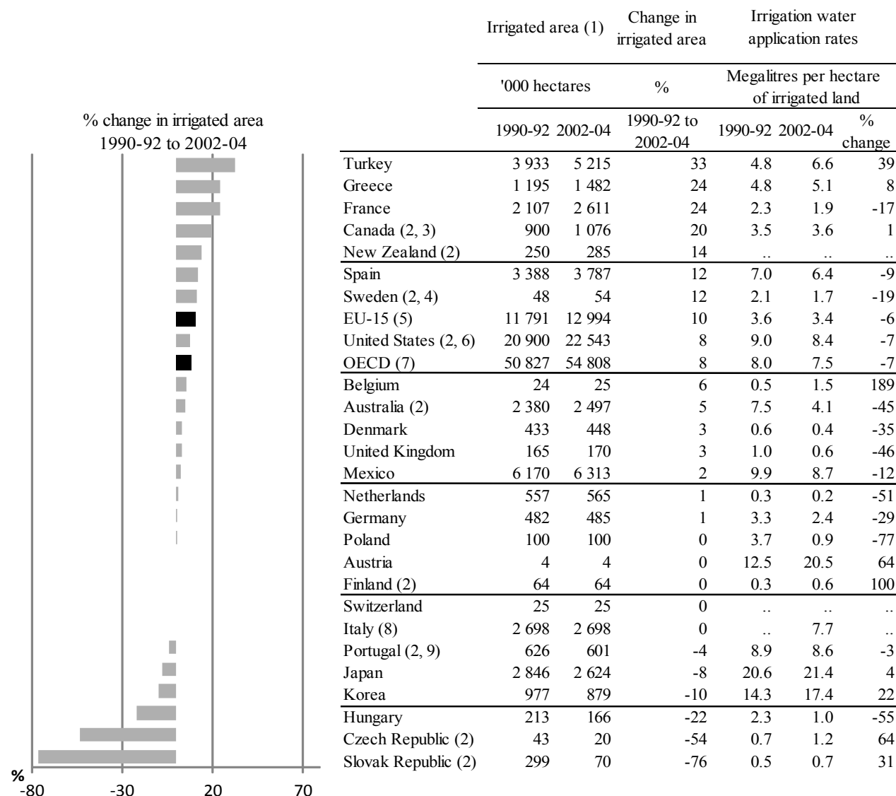
Figure 2. Irrigated area, irrigation water use and irrigation water application rates
