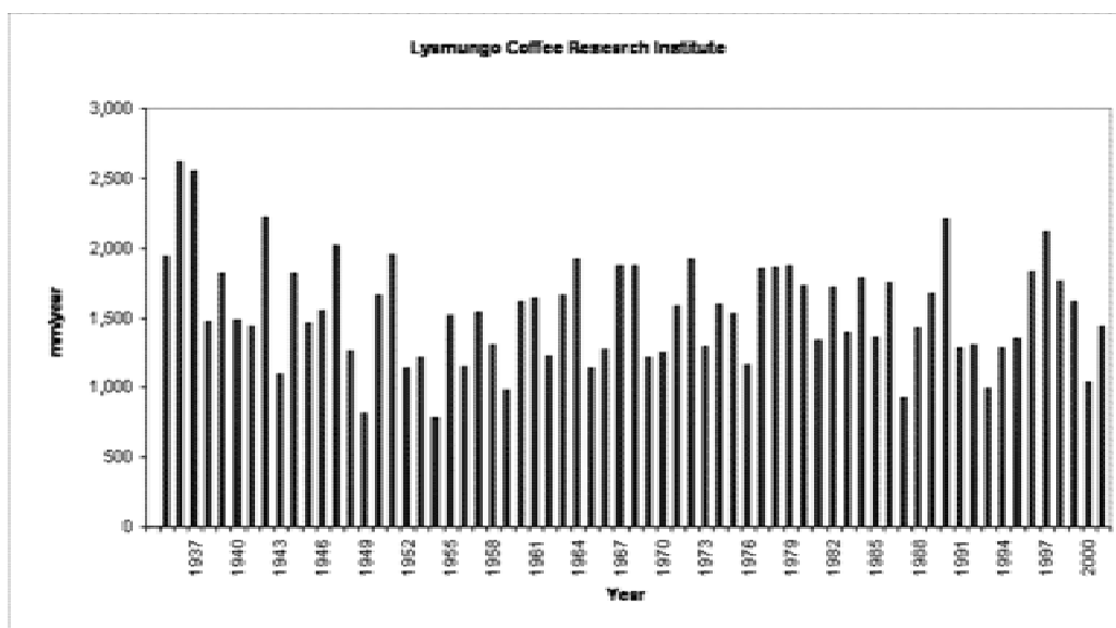
Figure 10. Annual precipitation at the Lyamungu Coffee Research Institute
