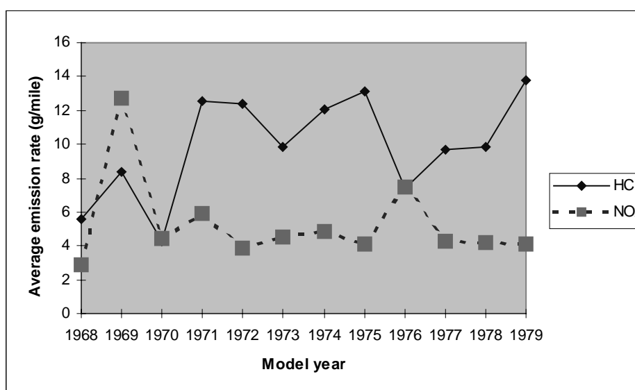
Figure 4 - Average emission rate (g/mile) by model year of the scrapped car, as measured by the Illinois EPA's pilot programme of 1992
