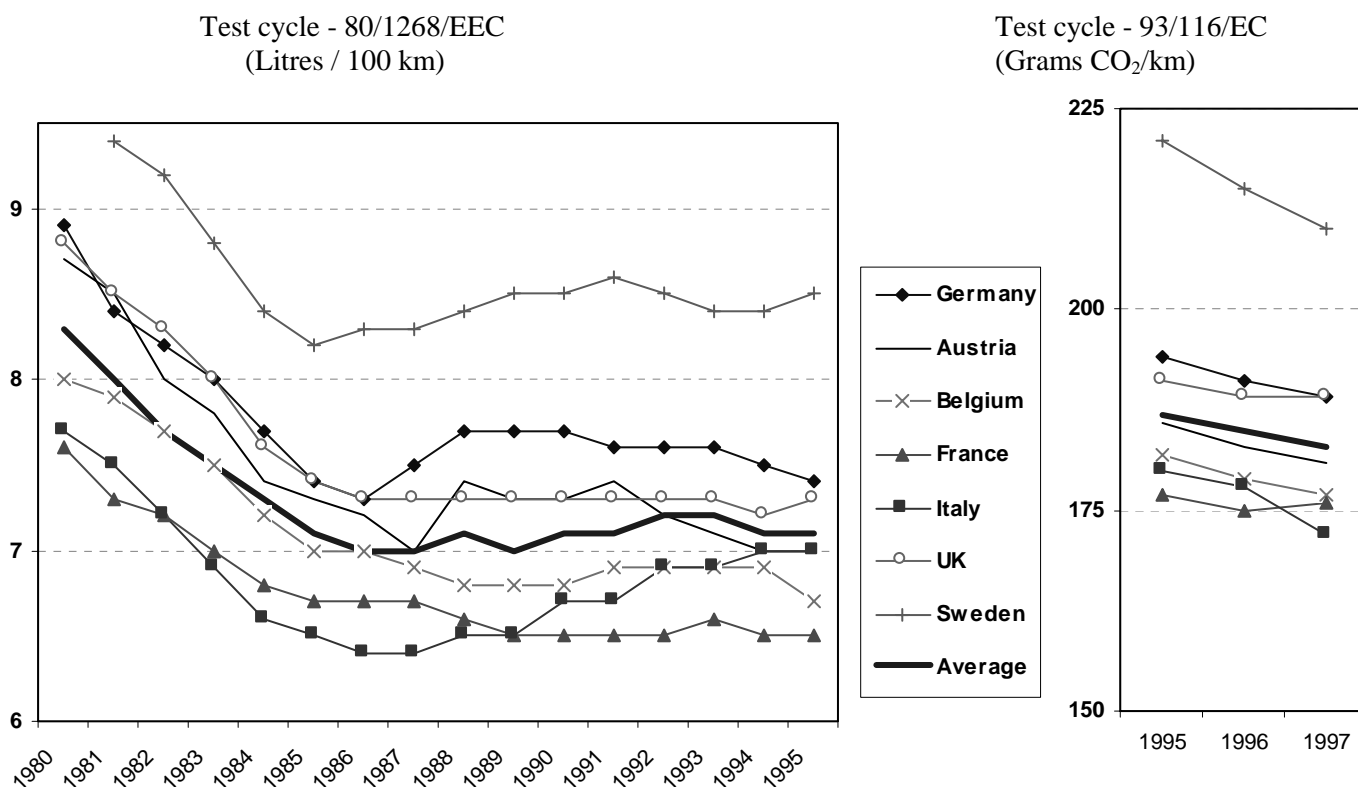
Figure 5 - Weighted Average Fuel Consumption and CO 2 Emissions, All New Cars
