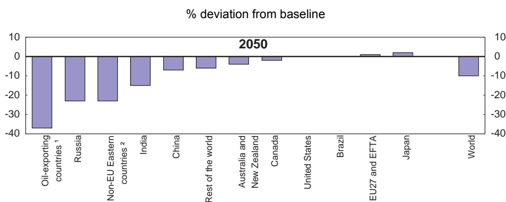
Figure 7. GHG emissions with fossil fuel subsidy removals
