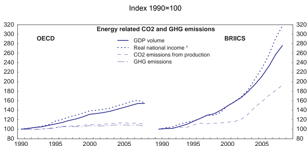
Figure 20. Decoupling trends – CO 2 emissions
