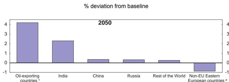
Figure 6. Impact of unilateral removal of fossil fuel subsidies on real income
